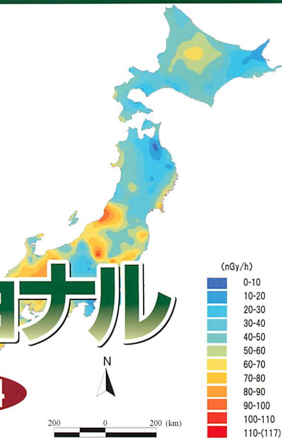
Distribution of the terrestrial gamma radiation dose rate in Japan
